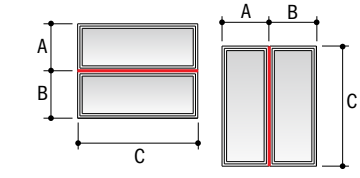
5 1/8" (130) x 3/4" (19) Fiberglass Joining Material For 4 7/8" (116) wall depth.
