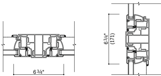
Horizontal Section Twin Casement
