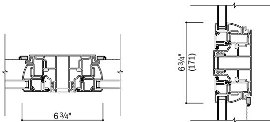
Horizontal Section Twin Casement
