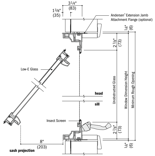
Vertical Section
